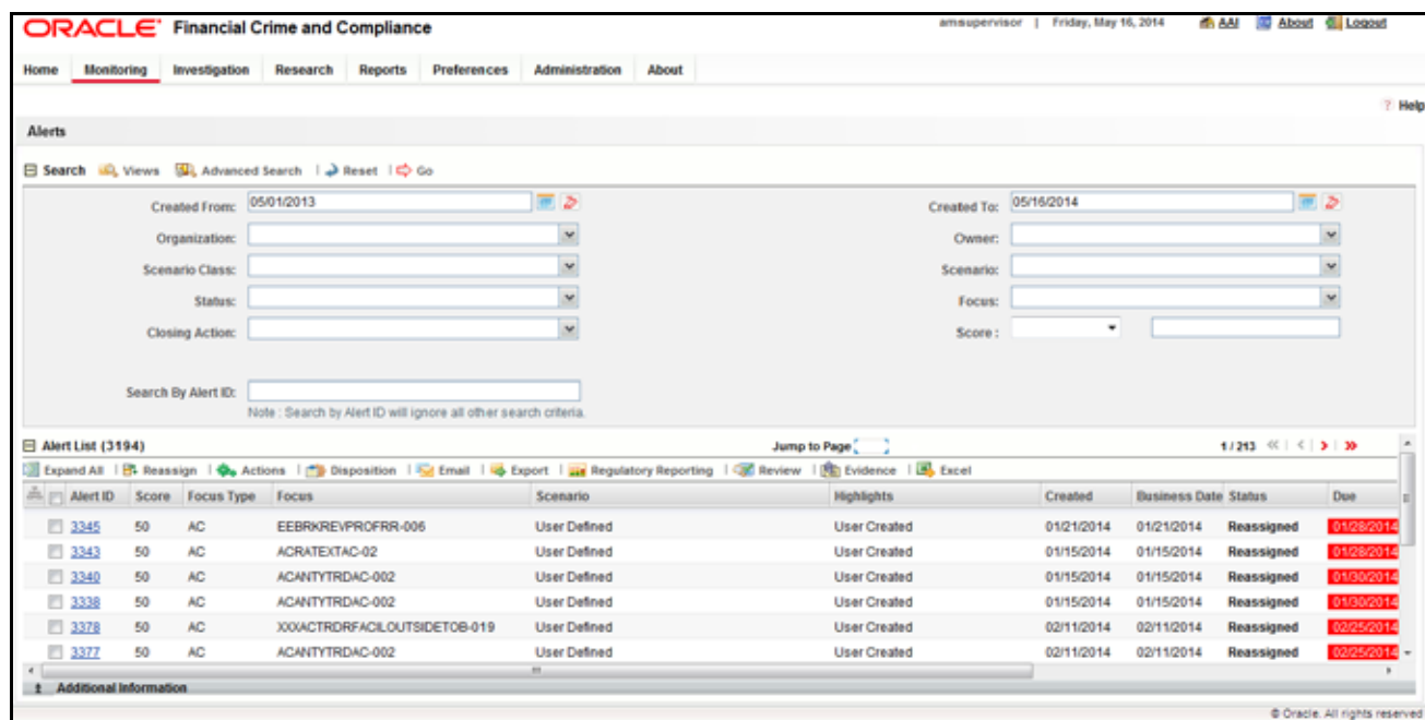
Figure 93. Navigation Features
